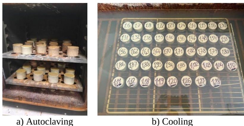
Figure 2 – Treatment of specimens
