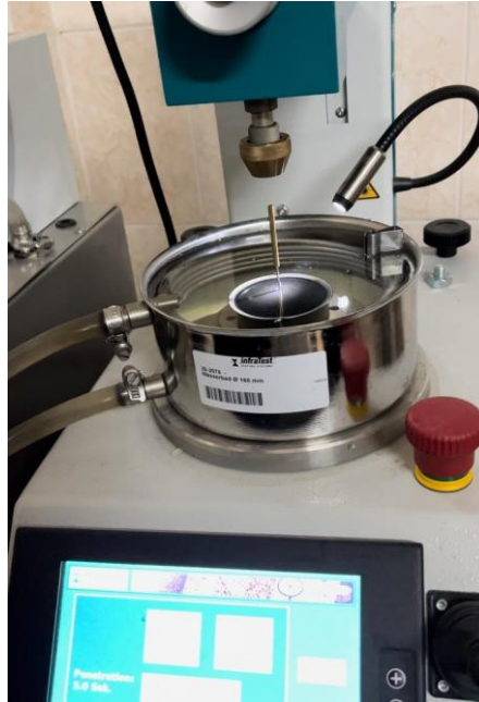
Figure 7 – Testing of the sample on the Infracast penetrometer
