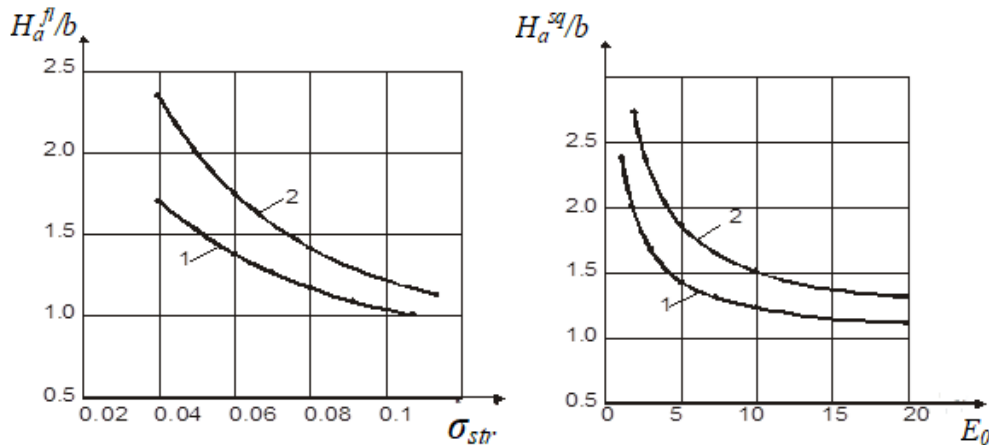
Figure 3 – The graph shows the relationship of the relative depth of the compaction deformation zone beneath foundation footings to the strength and deformation properties of the soil: a) The graph illustrates the dependency of the actual depth of the foundation compaction zone on the compressive strength of the soil's structural bonds; b) The graph depicts the relationship of the actual depth of the foundation compaction zone on the soil's deformation modulus
