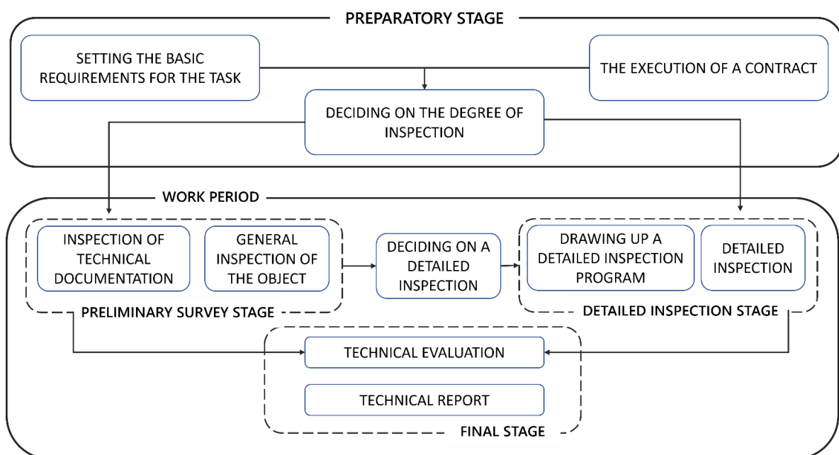
Figure 1 – Principle model of technical inspection
