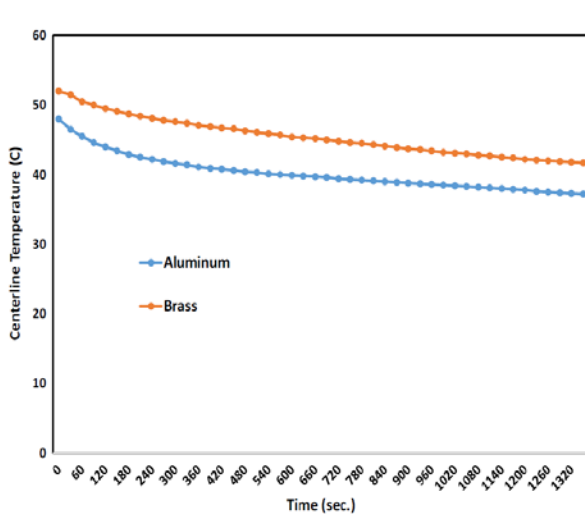
Figure 4 – Temperature ratio at the centerline of a cylindrical object at 52 °C in the atmosphere
