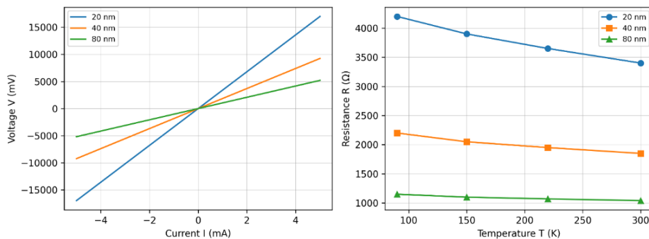
Figure 2 – DC transport characteristics of \text{Ni}_{80}\text{Cr}_{20} devices:
