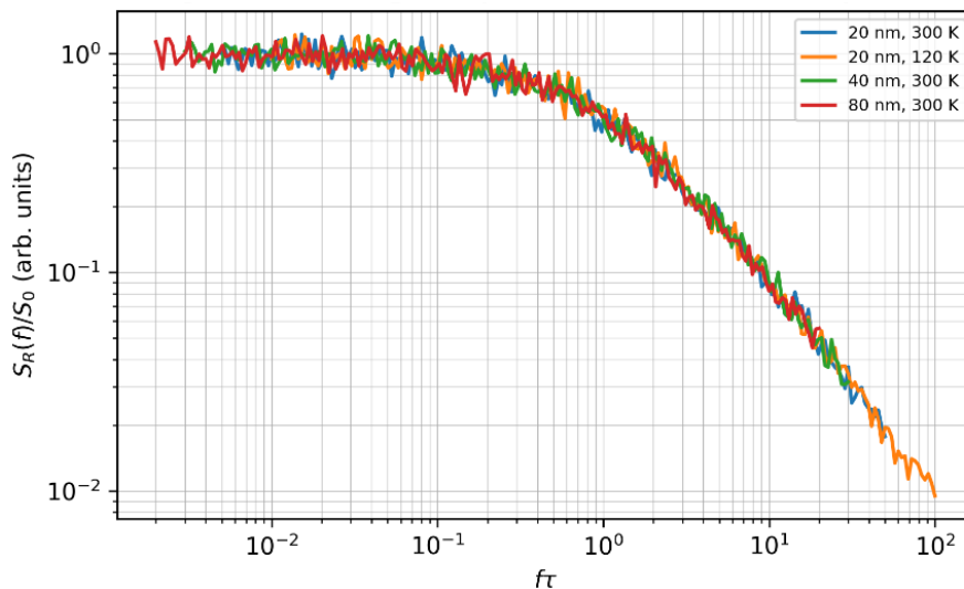
Figure 5 – Scaling collapse of normalized resistance noise spectra in \text{Ni}_{80}\text{Cr}_{20} films
