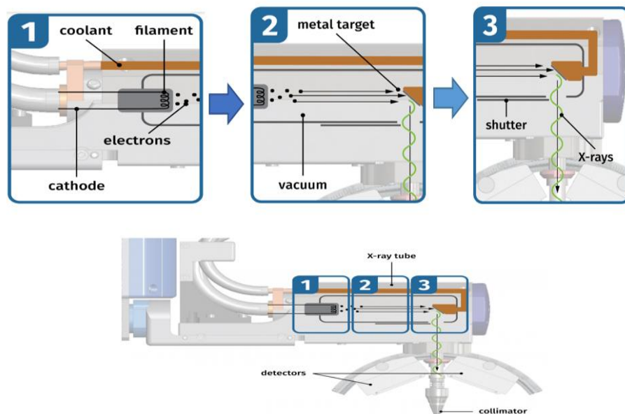
Figure 2 – Mechanism of X-ray generation
