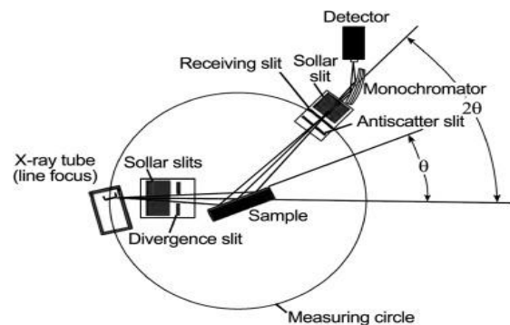
Figure 5 – Schematic diagram of HRXRD setup for epitaxial layer and interface analysis [17]
