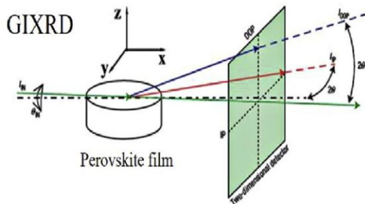
Figure 4 – GIXRD experimental setup [17]
