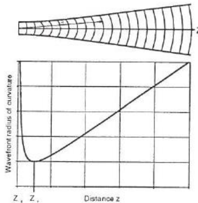
Figure 10 – Path of the wavefront's radius of curvature as a function of waist distance at z = 0
